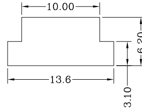
Panel hole dimensions
